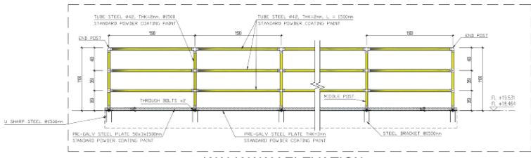
WALK WAY ELEVATION
